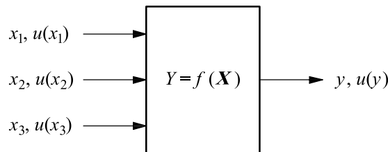
Figure 3 — Illustration of the law of propagation of uncertainty for N = 3 independent input quantities (5.4.4 and 5.6.3)
